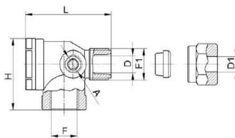
Raccordement F-Olive
